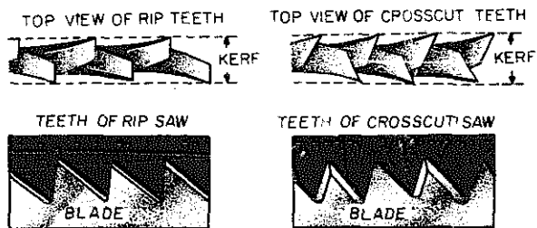
Figure 1-61.—Comparing rip and crosscut-saw teeth.
