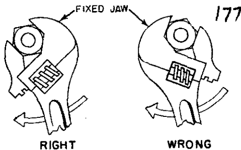
1.16.6(1) Figure 1-14.—Proper procedure for pulling adjustable wrenches.
