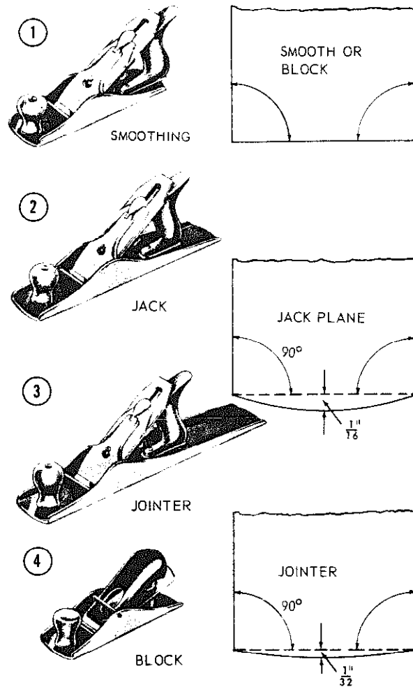
Figure 1-70.—Types of bench planes and block plane.
