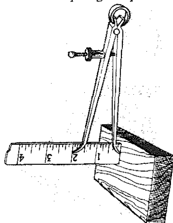
4.17H Figure 3-21.—Setting an inside spring caliper.
