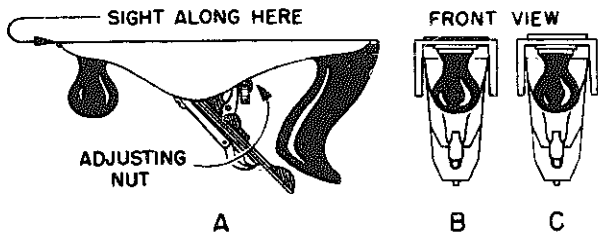
Figure 1-68.—Manipulation of the adjusting nut moves the plane iron up or down.
