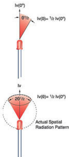
Fig. 6 - LED viewing angle
